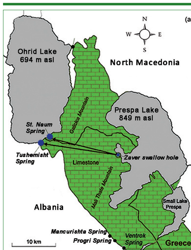
Fig. 1. Simplified hydrogeological map of the area between Prespa and Ohrid lakes
